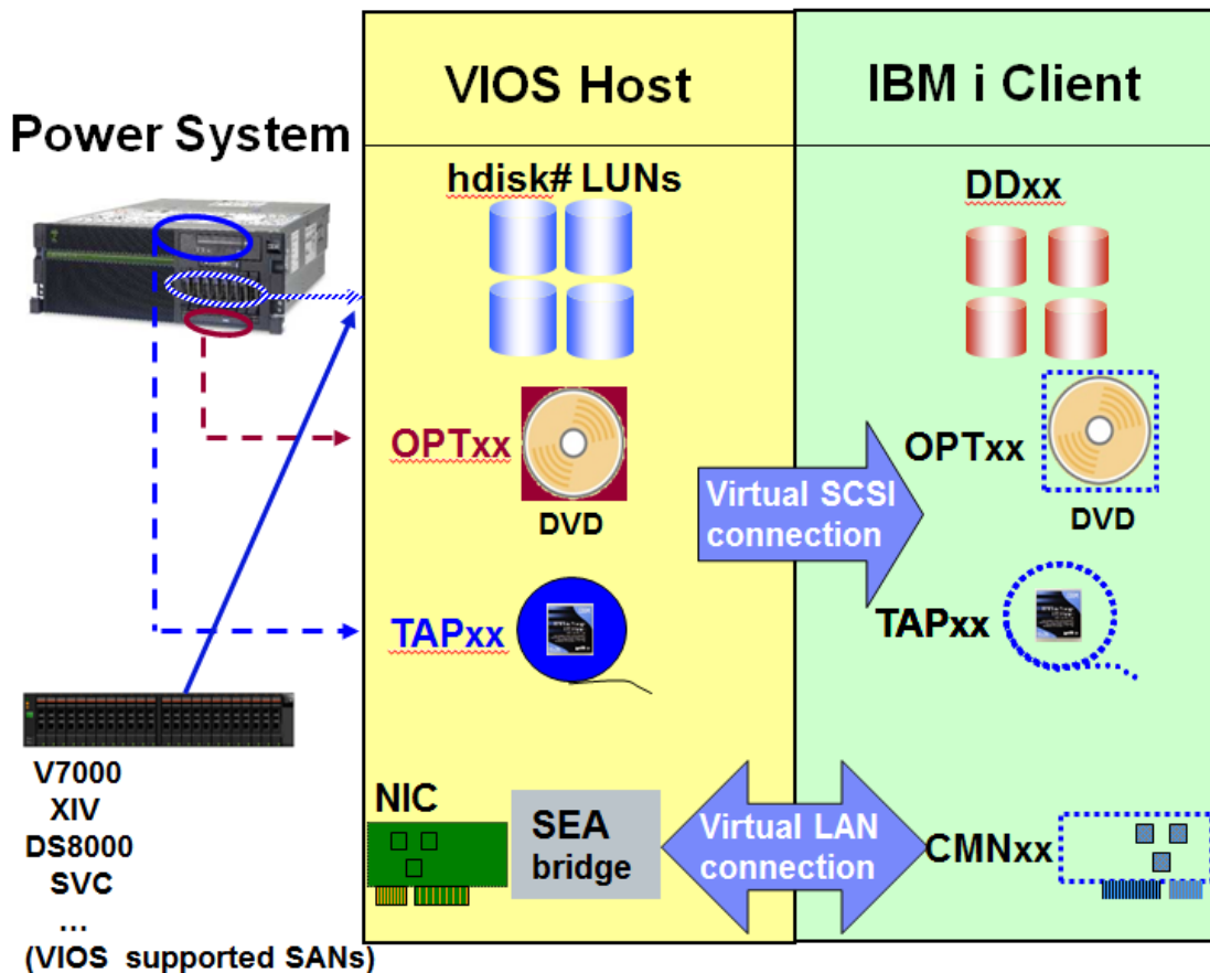
Figure 4: physical and virtualization components of the solution
