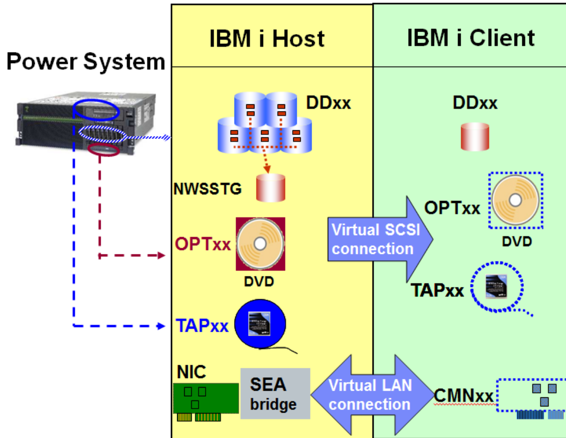
Figure 1: IBM i hosting IBM i components. Note: the IVE/Ethernet adapter represents a bridge that is configured from the virtual Ethernet LAN to a physical Ethernet port. It can also represent an IVE adapter with ports virtualized to the IBM i client partition.
