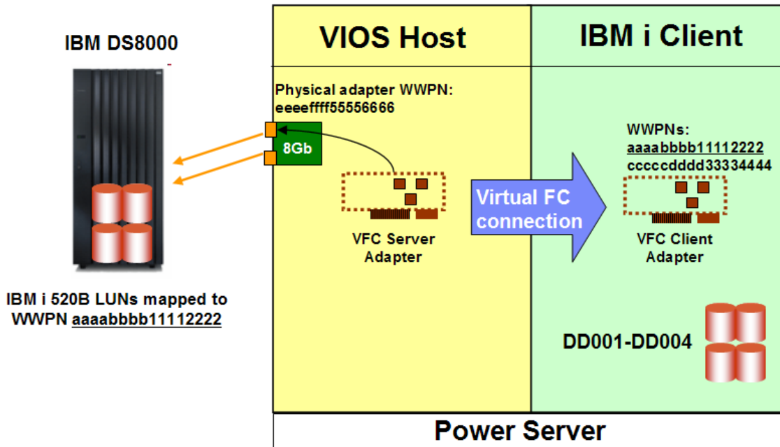
Figure 5: Using NPIV for IBM i
